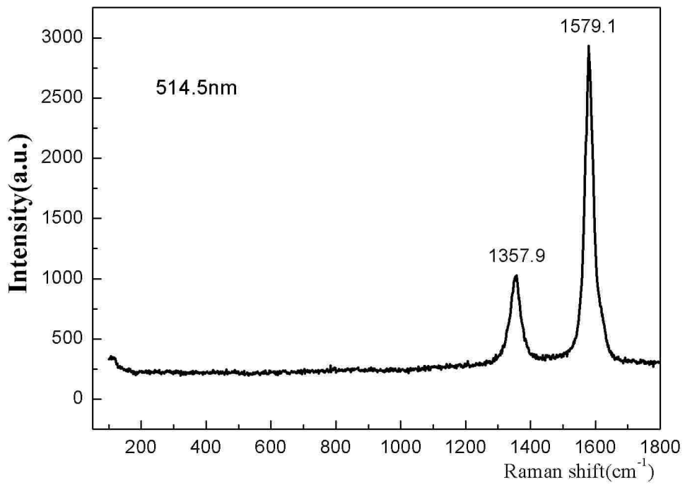
Raman spectrum of GM3
