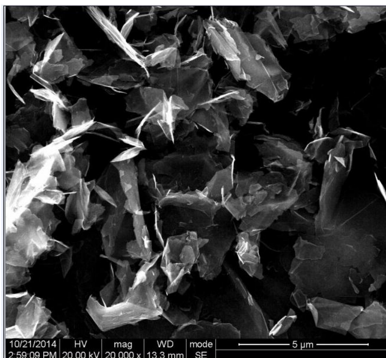
SEM of Industrial Graphite Nanoplatelet NMP Paste
