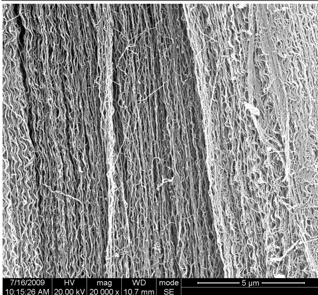
Transmission Electron Microscopy (SEM)
